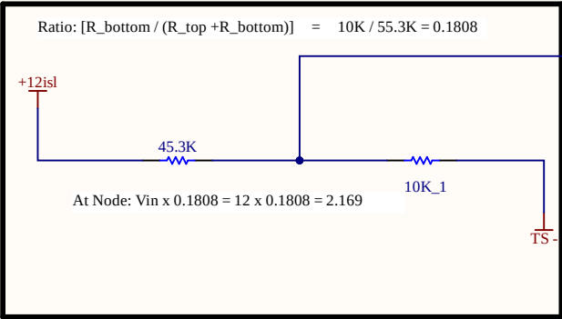
Reference Voltage (Half of TS Maximum [42V])
