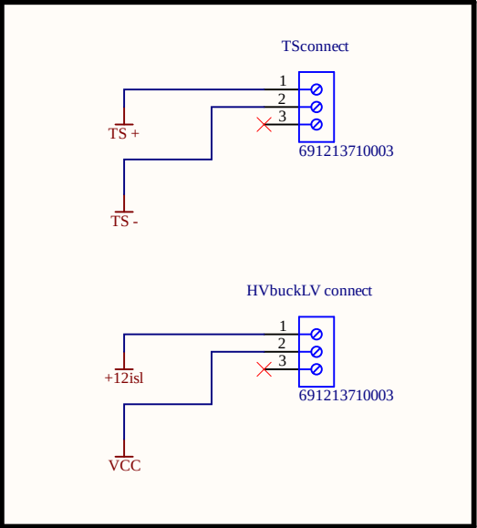
Input Connector
