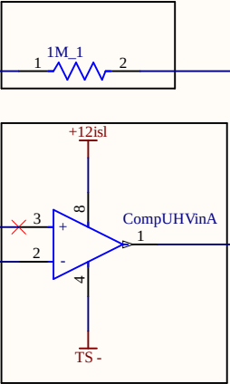
Hysteresis - (Voltage Difference between ON and OFF Voltage) ~ 0.11V
