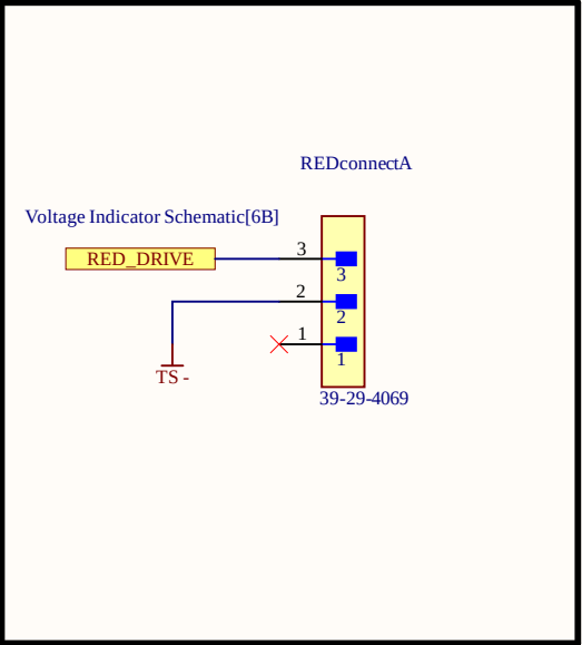
Output Connector
