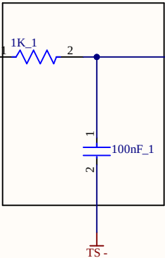
Ripple Filter
